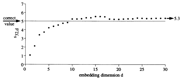
FIG. 7. Example of automatically fitted slopes s_{32,d} vs embedding dimension d for a typical reference point ( i=32 ). From embedding dimension d=18-30 the values of the slopes s_{32,d} show saturation and the average of the slopes s_{32,18}-s_{32,30} yields \langle s_{32} \rangle = 5.3 as an estimate for the pointwise correlation dimension.
